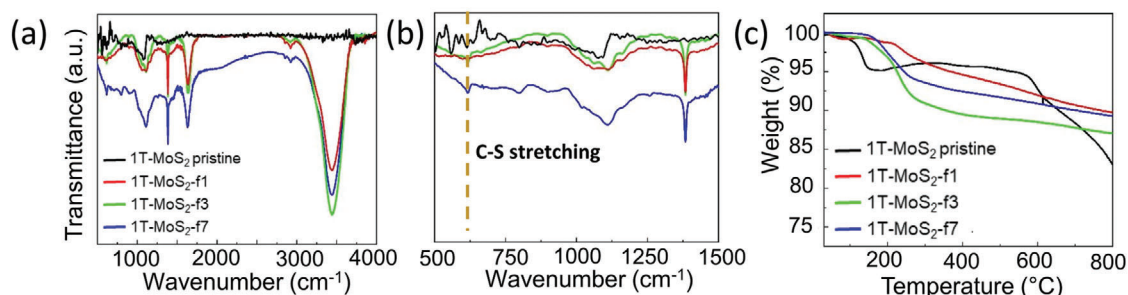
Figure 3. a) IR adsorption spectra of pristine and functionalized \text{MoS}_2 . (b) is a magnification of (a) in the range of 500\text{--}1500\text{ cm}^{-1} . c) TGA of pristine and functionalized \text{MoS}_2 .
