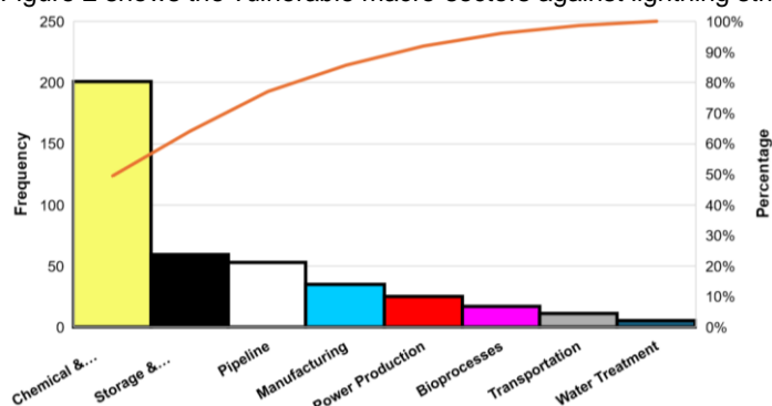
Figure 2: Pareto diagram for macro-sectors vulnerability against lightning strikes within the process industry.
