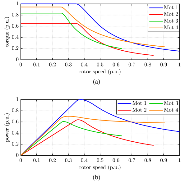
Fig. 2. Torque versus speed and power versus speed profiles of the four motors, normalized on the Mot1 specs.
