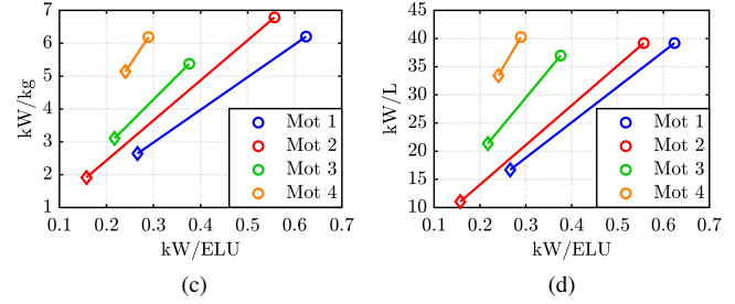
Fig. 10. Trade-off between torque and power densities (gravimetric and volumetric) and the specific torque and power per EPS
