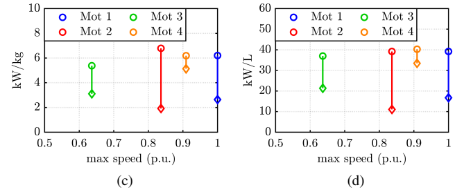
Fig. 6. Torque and power densities function of the maximum motor speed. Circle refers to peak condition and diamonds refers to max speed condition
