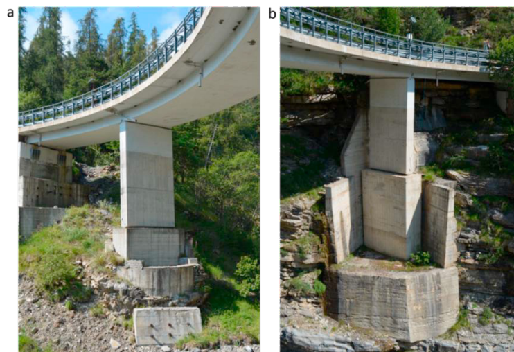
Fig. 1. Views of the Ponte Bavera bridge: (a) abutment and wall pier on Monesi side, (b) abutment and wall pier on Piaggia side.
