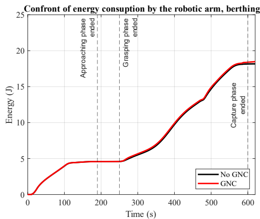
FIGURE 12: ENERGY CONSUMPTION OF THE ROBOTIC ARM DURING BERTHING MANEUVER
