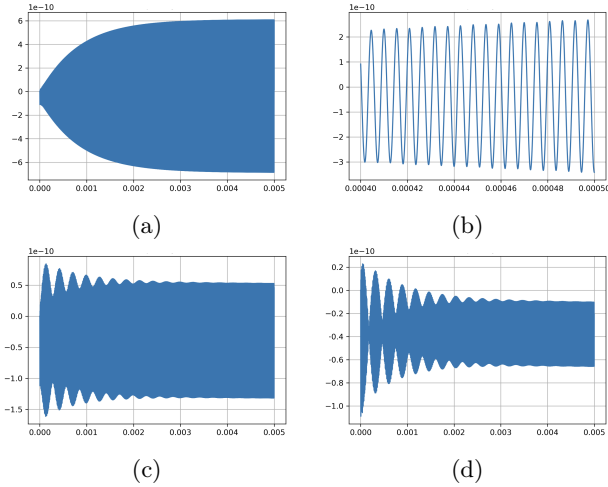
Figure 12: (a) Magnetic energy time trace for forced oscillator frequency at resonance, f_0 = 183.5 \text{ kHz} ; (b) same as in the previous panel, zoomed in the time interval between t = 0.4 \text{ ms} and t = 0.5 \text{ ms} . In (a) only the envelope of the fast oscillatory behaviour is evident, due to the time range of the plot. The envelope of the oscillatory behaviour of the magnetic energy is shown for off-resonant frequencies of the forced oscillator in (c) for f_0 = 180 \text{ kHz} and (d) for f_0 = 187 \text{ kHz} .
