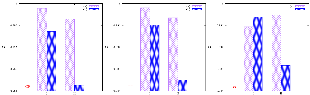
Fig. 12. Variations of the dimensionless natural frequency relative to along-the-width symmetric size increment of debonding for CF, FF, and SS boundary conditions in bending modes.
