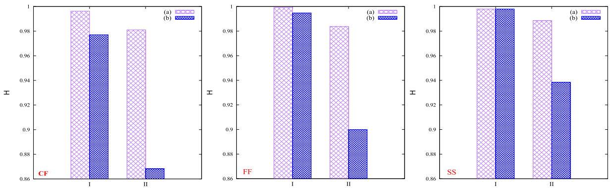
Fig. 11. Variations of the dimensionless modal loss factor relative to along-the-width symmetric size increment of debonding for CF, FF, and SS boundary conditions in bending modes.
