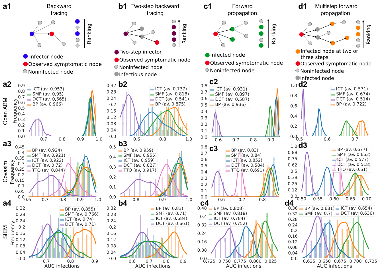
Fig. 4. Detection of the one-step, two-step backward, one-step, multistep forward tracing. Panels (a.1), (b.1), (c.1), and (d.1) show a schematic representation of the one-step, two-step backward, one-step, and multistep forward transmissions respectively. See the main text for a formal definition. The second, third, and fourth rows show the histogram of the AUC associated with the detection of the four types of infected individuals, for OpenABM, Covasim, and StEM, respectively. The methods used to obtain the ROC curves are Belief Propagation (BP), Simple Mean Field (SMF), Informed Contact Tracing (ICT), DCT, and Trace-Test-Quarantine (TTQ). The simulation set-up used for these results is the same exploited for the detection of the superspreaders illustrated in Figure 3. The average AUC is reported in the legend for the methods, while the lines report kernel density estimates to guide the visualization of the histograms.
