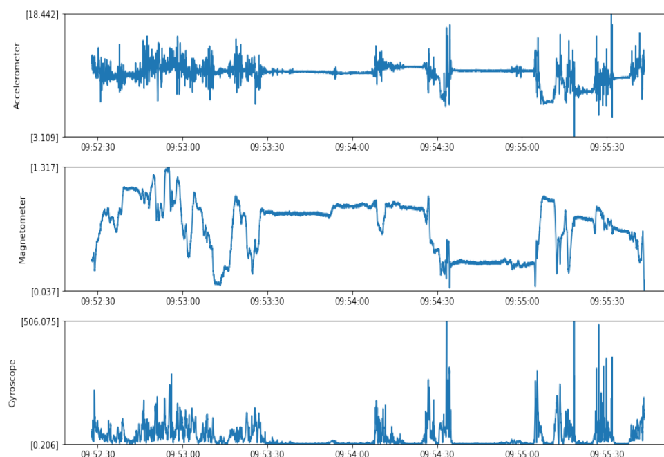
Figure 2. Accelerometer, magnetometer, and gyroscope sample magnitude data before preprocessing.
