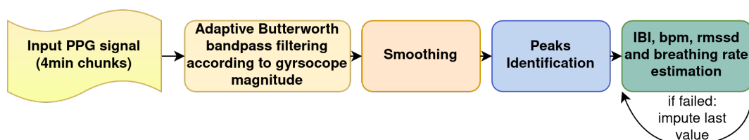
Figure 5. Preprocessing of the PPG signal and the extraction of features.
