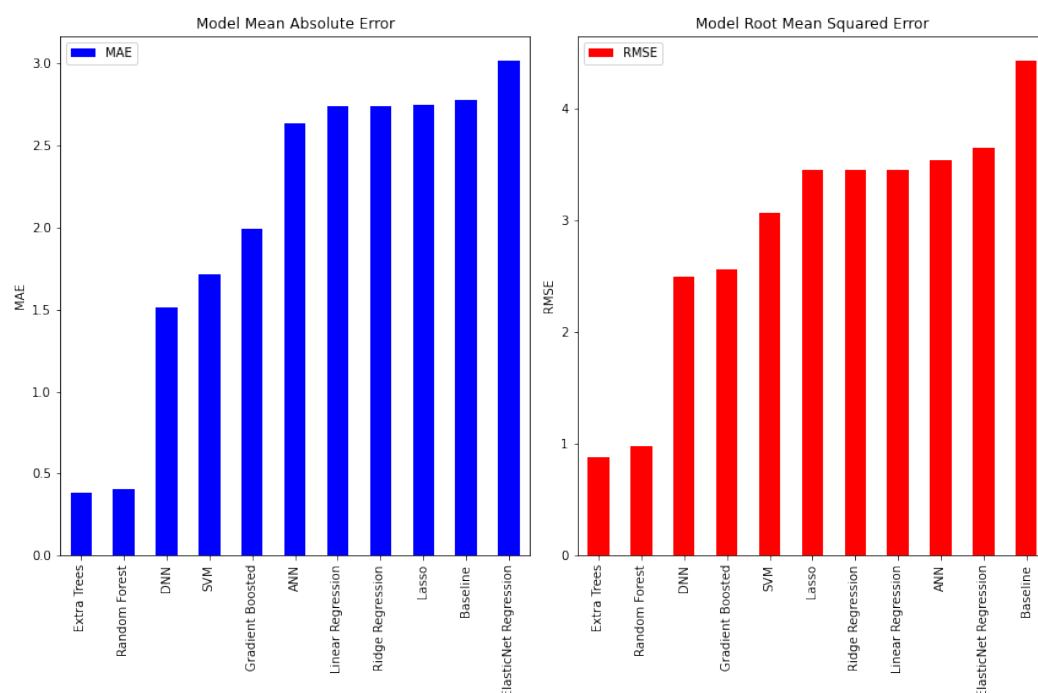
Figure 8. Comparison of machine learning techniques in terms of the MAE and RMSE for FEAT1.
