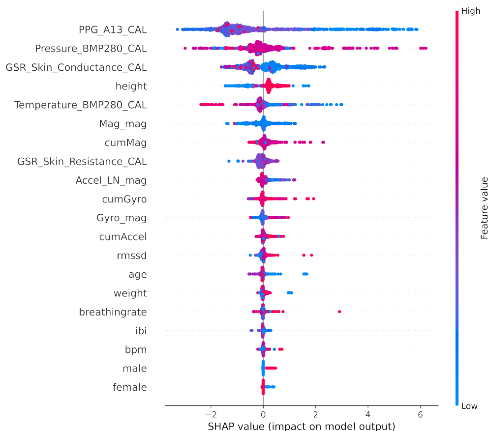
Figure 9. Shapley values for the random forest model using SHAP to show the impact of each feature on the model output (please refer to Table 2 for the meaning of the features).
