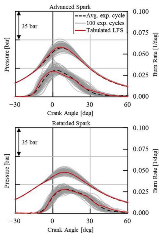
Fig. 13. Experimental (black dashed) and predicted (red) average in-cylinder pressure and burn rate; 100 experimental consecutive cycles (grey). Two different spark timings at same lambda, boost pressure and EGR (partial load). (For interpretation of the references to color in this figure legend, the reader is referred to the Web version of this article.)
