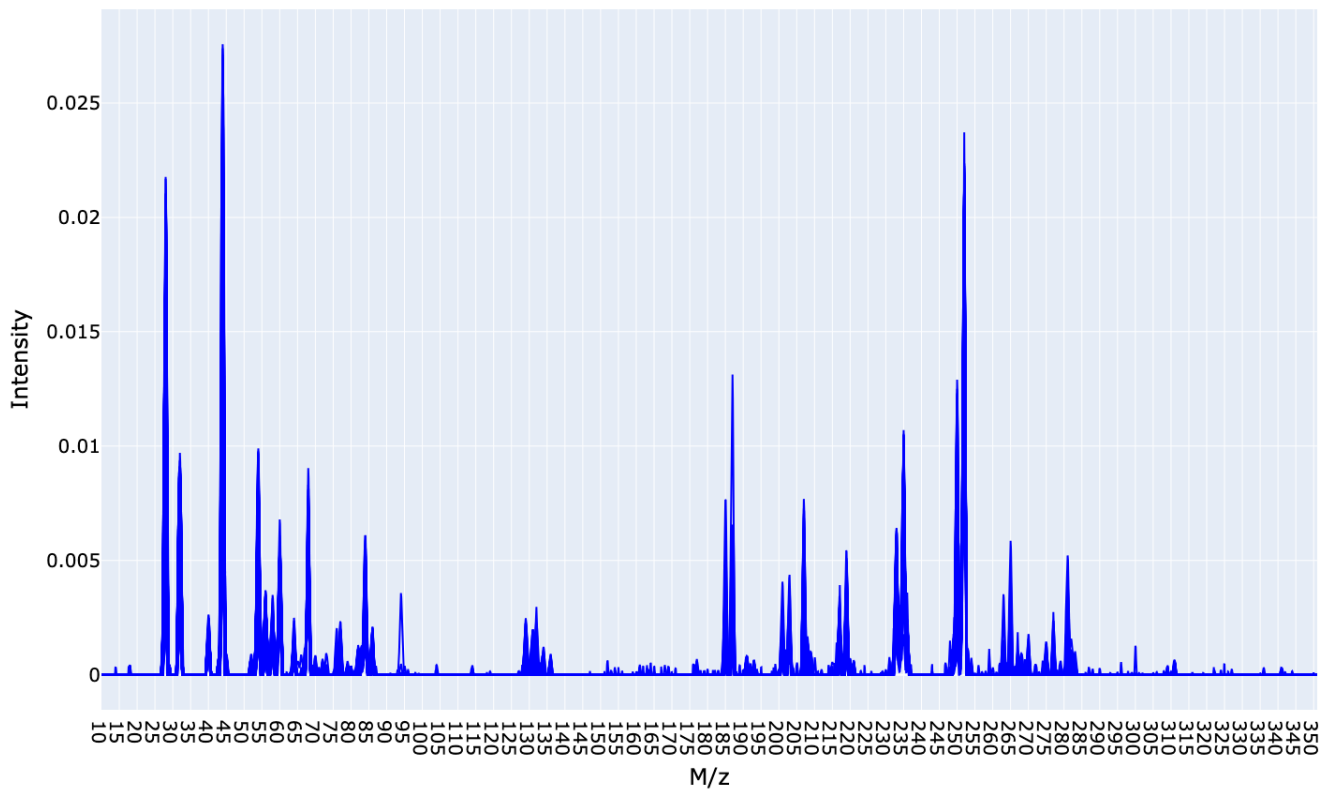
Whole mass spectra, normalized and filtered (Positives)
