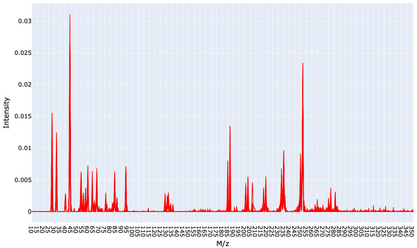
Figure 5. Examples of whole spectra (10 m/z to 351 m/z) for negative subjects (top, blue) and positive ones (bottom, red)
