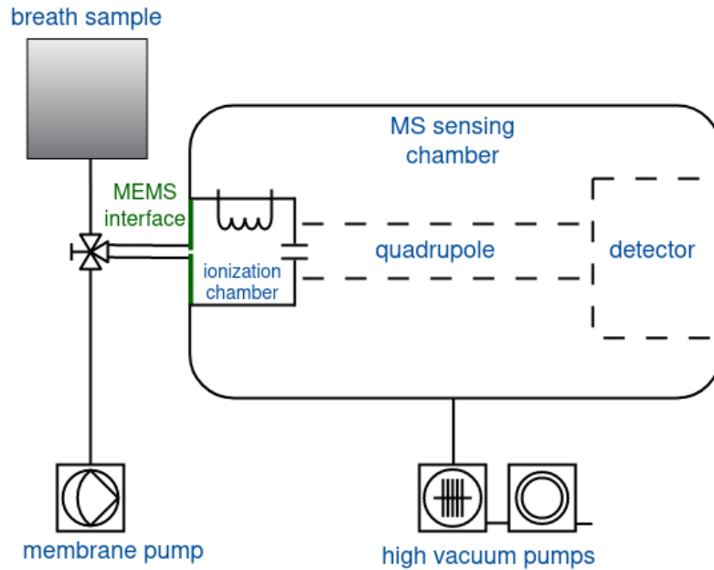
Figure 1. Schematic of the Mass Spectra analyzer
