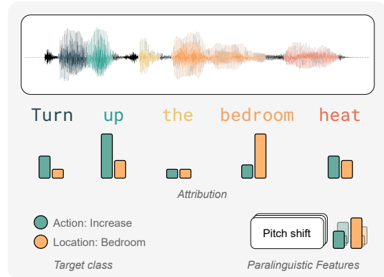
Figure 1: Explanation with word-level and paralinguistic attributes for a Fluent Speech Commands sample (Lugosch et al., 2019). Audio aligned to words represented through color. Bars show word-level attributions for target classes Increase (green) and Bedroom (orange).
