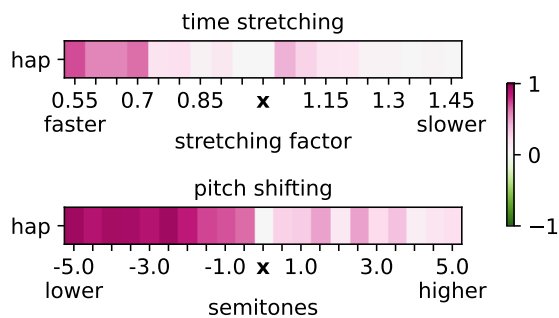
Figure 5: r_p(\tilde{\mathbf{x}}) breakdown for p := time stretching, and pitch shifting; same instance \mathbf{x} of Table 5.
