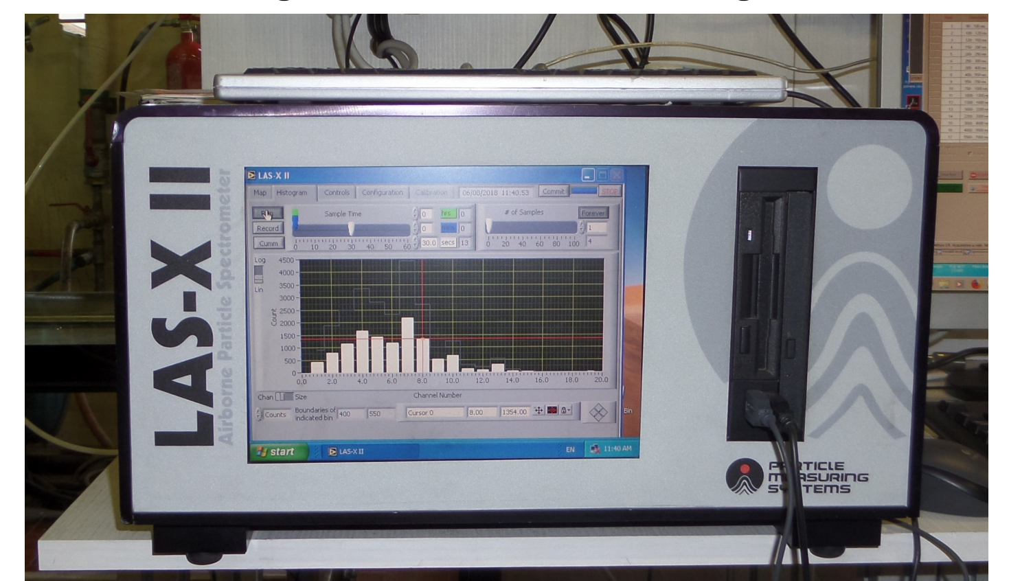
Figure 6. Particle spectrometer.
