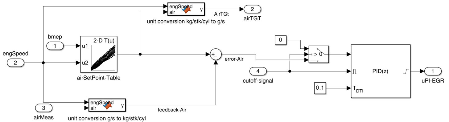
Figure B2. EGR control, closed loop branch
