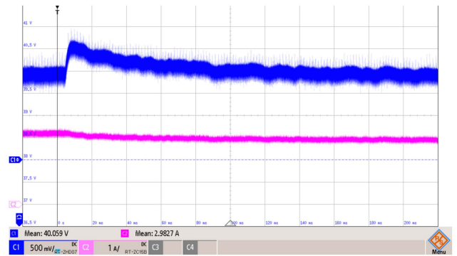
FIGURE 20. Experimental data recorded with the oscilloscope during the disturbance rejection of an increase of 10 Ω in VL.
