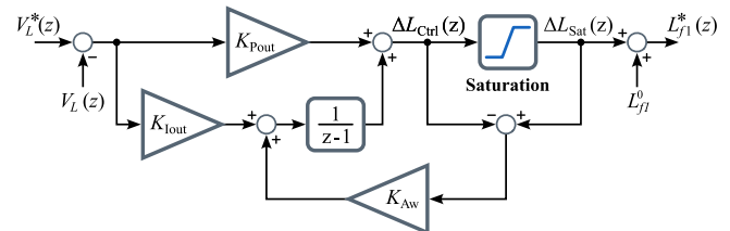
FIGURE 10. Proposed control scheme for the outer Loop.
