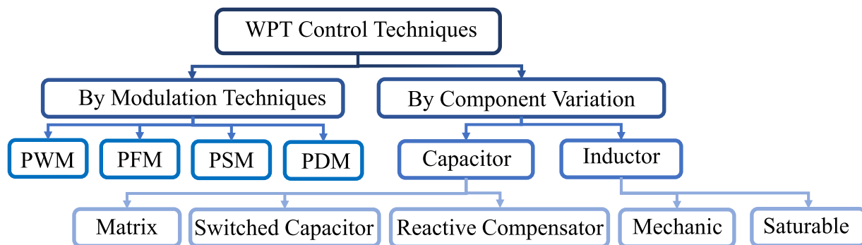
FIGURE 1. Classification of control techniques for WPT systems.
