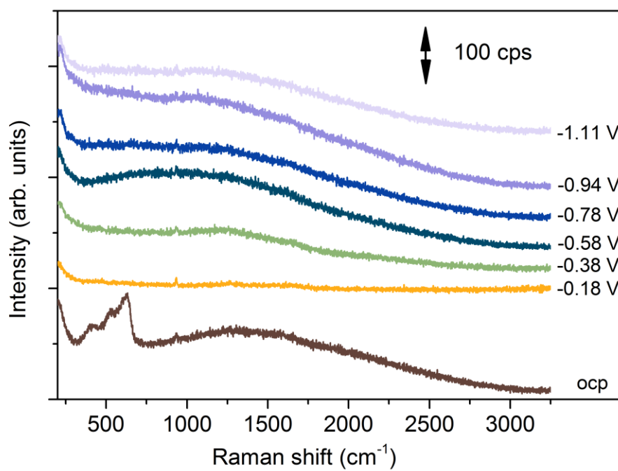
Supplementary Figure 8. Electrochemical Raman spectra of the electrochemically-polished Cu foil electrodes at potentials from OCP to -1.11 V_{\text{RHE}} in an Ar-saturated 0.1 M \text{NaClO}_4 solution.
