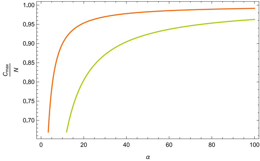
Fig. 6. HIT \frac{C_{\max}}{N} of a heterogeneous population, for R_0 = 2.5 , as a function of \alpha in the case of a two-parameter gamma distribution, for two different values of \eta . The orange curve originates from taking \eta = 2 , while the green one from \eta = 9 .
