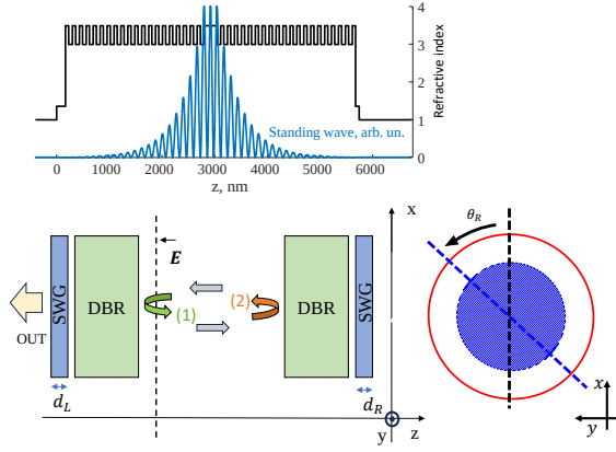
Fig. 1. Top: Refractive index and standing wave profile of our VCSEL structure. The structure designed for a wavelength of 850 nm features a \lambda -cavity, two symmetric 20-pairs \lambda/4 DBRs terminated by sub-wavelength surface gratings (SWGs). The high and low values of refractive index are chosen to be n_H = 3.5 and n_L = 3 , respectively. Bottom: Schematics of the cavity to be investigated within the Barkhausen round-trip cavity framework with the orientation of the tilted gratings (right).
