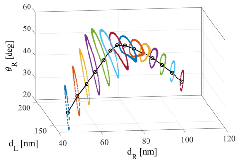
Fig. 4. Circular polarization design chart. S_3=1 trajectory (Iso-Circular-Polarization line) in the 3D parameter space and the regions featuring S_3 \geq 0.99 within the colored lines.
