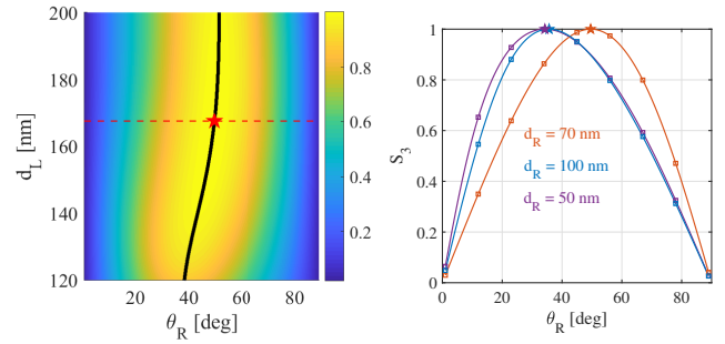
Fig. 3. Left: Color density plot of S_3 vs. d_L and \theta_R for d_R=70 nm. The red dashed line is the cut at the d_L grating thickness that ensures S_3=1 ( S_3 = 1 at the star). The black line is the \theta_R at which the S_3 is the maximum for each d_L value. Right: S_3 vs. \theta_R for three values d_R = 50, 70 and 100 nm. The red curve is the cut on the left for d_L = 167 nm. Similarly, for maps computed for d_R=50 and 100 nm, we observe S_3=1 (stars) for d_L=141 and 199 nm. The squares represent the values obtained with VELMS-1D.
