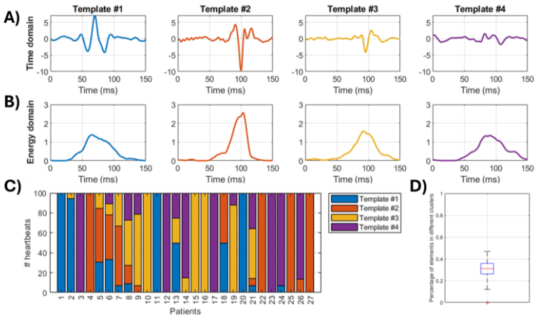
Figure 3. Templates identified for S2 in the time (A) and energy (B) domains, distribution of the templates over each patient’s heartbeats (C), and boxplot of heartbeats clustered differently over 100 repetitions (D).
