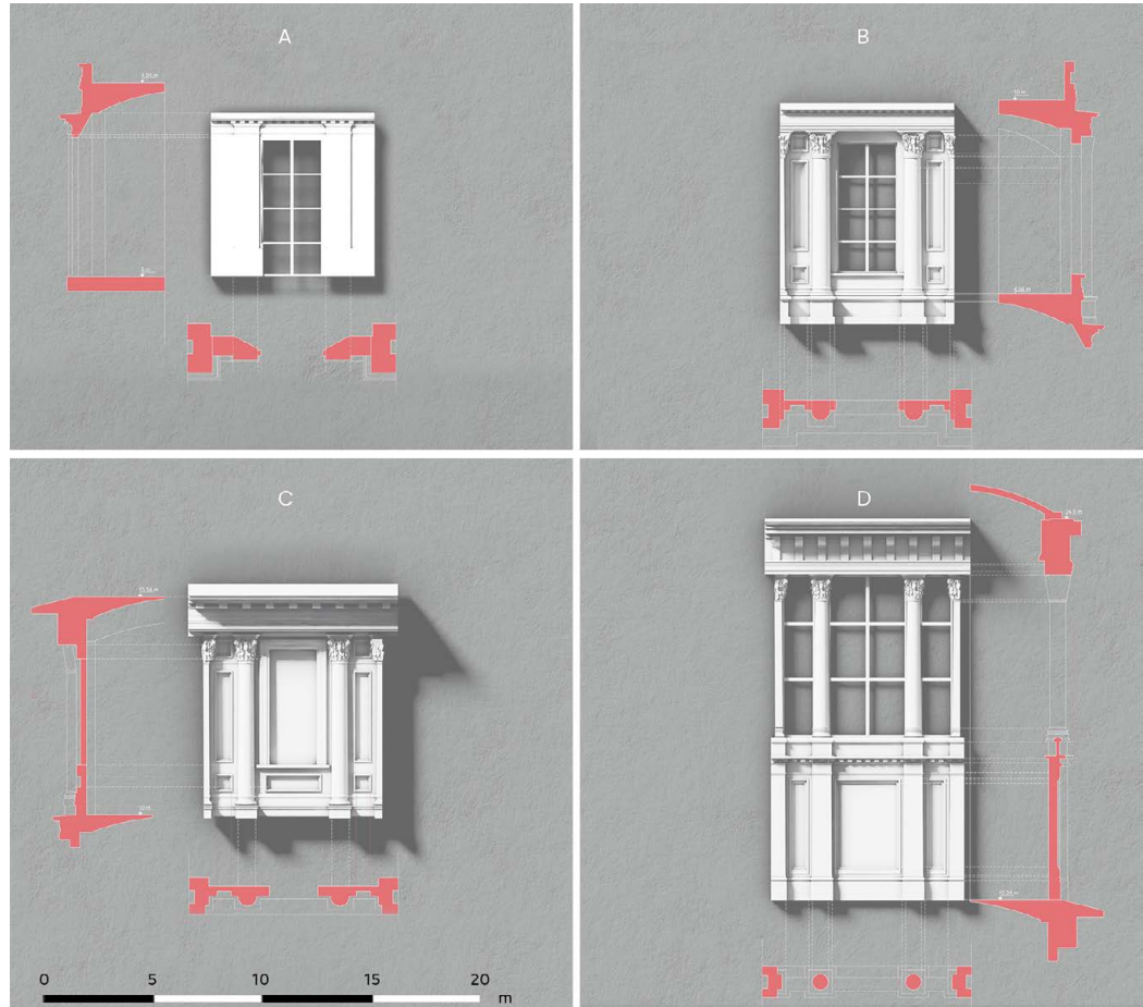
Fig. 8. Object-based matrix parts of a “dynamic model” facade. Elaboration by L. Torresi.
