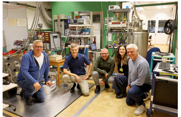
Fig. 1. METAS laboratory with the authors and the three installed bridges: from left to right, METAS DJIB, CMI FDIB, INRIM-POLITO FDIB.
