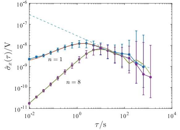
Fig. 2. Calculated (solid lines) and measured Allan deviations of the DUT X channel for the filters of order 1 and 8 (the parameters are given in the text), when the input is driven by white noise. The dashed line represents the Allan deviation of the unfiltered white noise.
