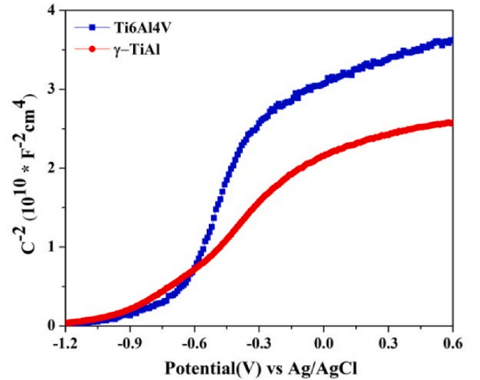
Fig. 4. Mott-Schottky curves at frequency 1 kHz measured in the cathodic direction for EB-PBF-produced Ti6Al4V and \gamma -TiAl alloy for 1 h in 0.9 % NaCl solution.
