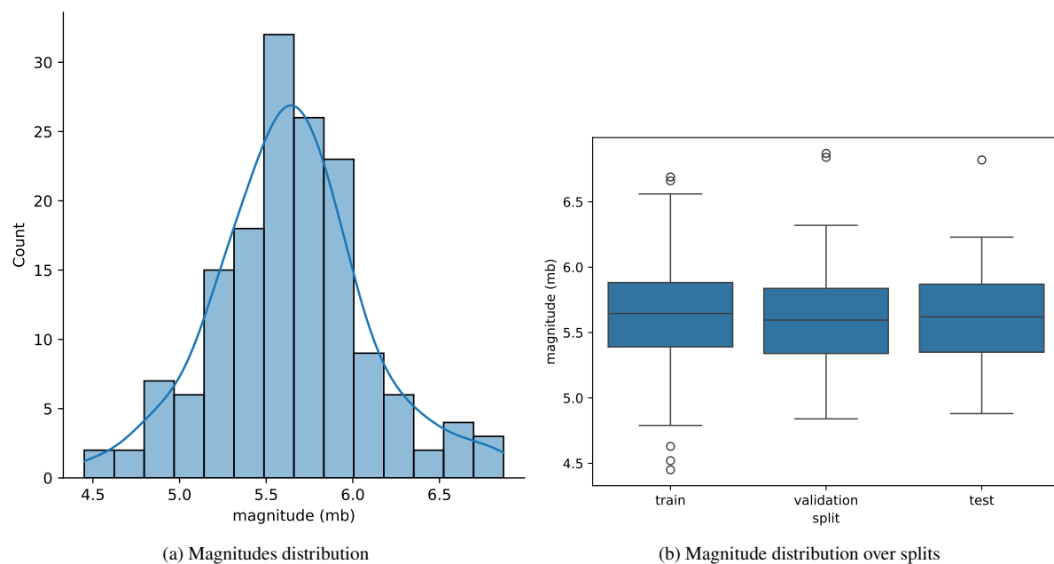
Figure 3. Magnitude distributions
