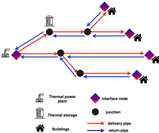
Fig. 2. Example of a DH network.
