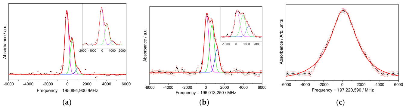
Figure 4. \text{Er}^{3+} absorption spectra and their fitting of sample \text{Er:LiYF}_4 100 ppm for (a) ^4\text{I}_{15/2} \Gamma_{56}^{(1)} \rightarrow ^4\text{I}_{13/2} \Gamma_{78}^{(1)} ; (b) ^4\text{I}_{15/2} \Gamma_{56}^{(1)} \rightarrow ^4\text{I}_{13/2} \Gamma_{56}^{(1)} ; (c) ^4\text{I}_{15/2} \Gamma_{56}^{(1)} \rightarrow ^4\text{I}_{13/2} \Gamma_{78}^{(2)} . The red line is the total nonlinear fitting, the magenta, green and blue lines are the individual peaks that contribute to the convolution.
