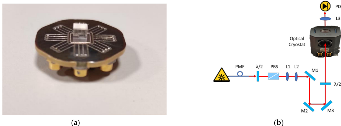
Figure 1. (a) A picture of sample ^{166}\text{Er}:\text{LiYF}_4 100 ppm. (b) Measurement setup. PMF: polarization-maintaining fiber; L: lens; M: mirror; \lambda/2 : polarization rotator; PBS: polarization beam splitter; PD: photodiode. The blue lines represent the optical fiber path, and the red ones represent the free space path.
