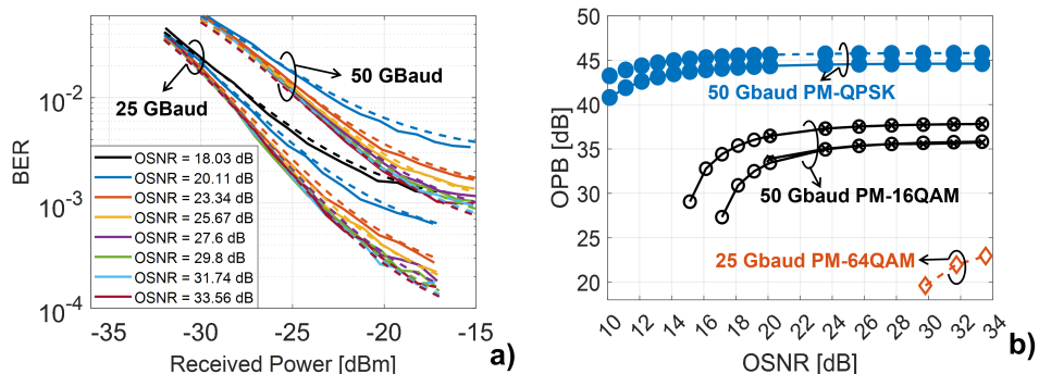
Fig. 3: a) Experimental (solid) and analytical (dashed) BER vs P_{RX} at different OSNR_{metro} for 25 and 50 GBaud PM-16QAM. b) OPB vs OSNR_{metro} at BER = 10^{-2} (solid) and 2 \cdot 10^{-2} (dashed) for analytical 50 GBaud PM-QPSK (blue, dots), analytical (circles) and experimental (crosses) 50 GBaud PM-16QAM (black) and analytical 25 GBaud PM-64QAM (orange, diamonds).
