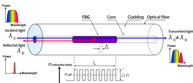
Figure 2 Working principle of FBG.
