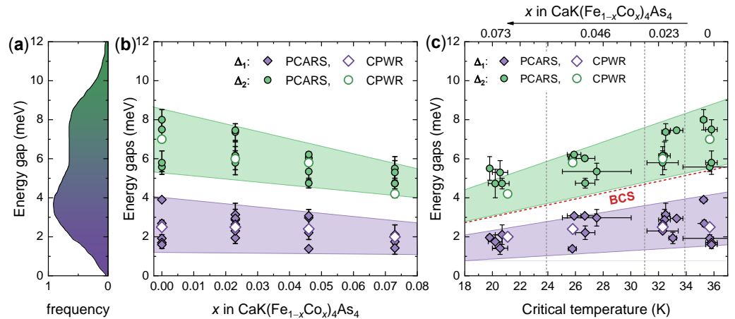
Figure 4. Doping and critical temperature dependence of the superconducting gaps in CaK(Fe 1-x Co x ) 4 As 4 single crystals. (a) An example of the distribution of gap amplitudes obtained by STM in the pristine compound (taken from Ref. [25]), which is in very good agreement with the results obtained by PCARS and CPWR in crystals with x = 0 . (b) Gap amplitudes \Delta_1 and \Delta_2 as a function of the doping content x . Error bars on the PCARS data indicate the range of gap values obtained by fitting the same curve with different normalizations, and symbols indicate the midpoint of this range. Colored regions are just guides to the eye and highlight a linear-with-doping suppression in both the gap amplitudes. (c) Energy gaps as a function of the critical temperature of the contacts (PCARS) or of the critical temperature where the superfluid density goes to zero (CPWR). The meaning of vertical error bars is the same as in (b), while horizontal error bars indicate the uncertainty on the critical temperature. Colored regions are bounded by lines corresponding to constant gap ratios 2\Delta_i/k_B T_c . The dashed red line corresponds to the BCS gap ratio 2\Delta/k_B T_c = 3.53 . The Co content to which the points refer is indicated on top of the panel and increases from right to left.
