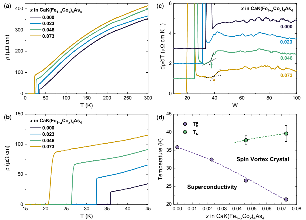
Figure 1. Electric transport in \text{CaK}(\text{Fe}_{1-x}\text{Co}_x)_4\text{As}_4 single crystals. (a) In-plane resistivity \rho as a function of temperature T for an undoped sample ( x = 0 ) and three samples with increasing Co doping ( x = 0, 0.023, 0.046 , and 0.073 ). (b) Low- T magnification of (a) which highlights the onset of superconductivity. The transition temperature T_c^\rho is defined as the midpoint of each resistive transition. (c) T dependence of d\rho/dT obtained by numerical derivation of the curves shown in (a). Arrows highlight the step-like increase associated with SVC magnetic ordering at the Néel temperature T_N , as estimated by the intersection of the linear fits above and below T_N (dashed black lines). The curves are vertically offset for clarity. (d) T - x phase diagram determined from transport measurements. Data points for T_c^\rho and T_N as a function of x mark the boundaries of the two main ordered phases, superconductivity and SVC magnetic order. Dashed lines are guides to the eye.
