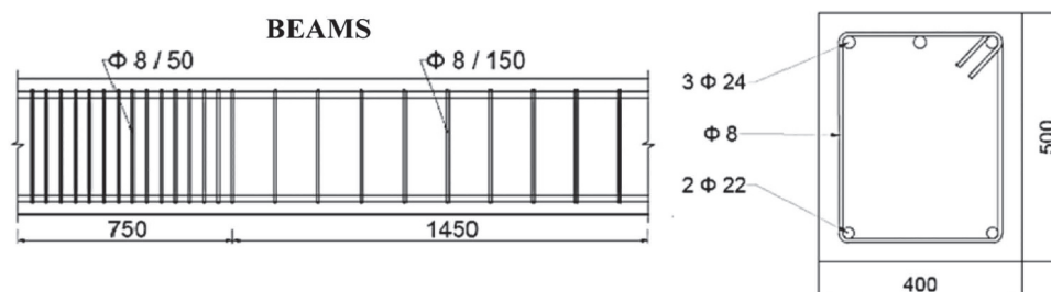
Fig. 3. Proposed seismic design: stirrups with the cross-section of the beams. Measurements in millimetres.
