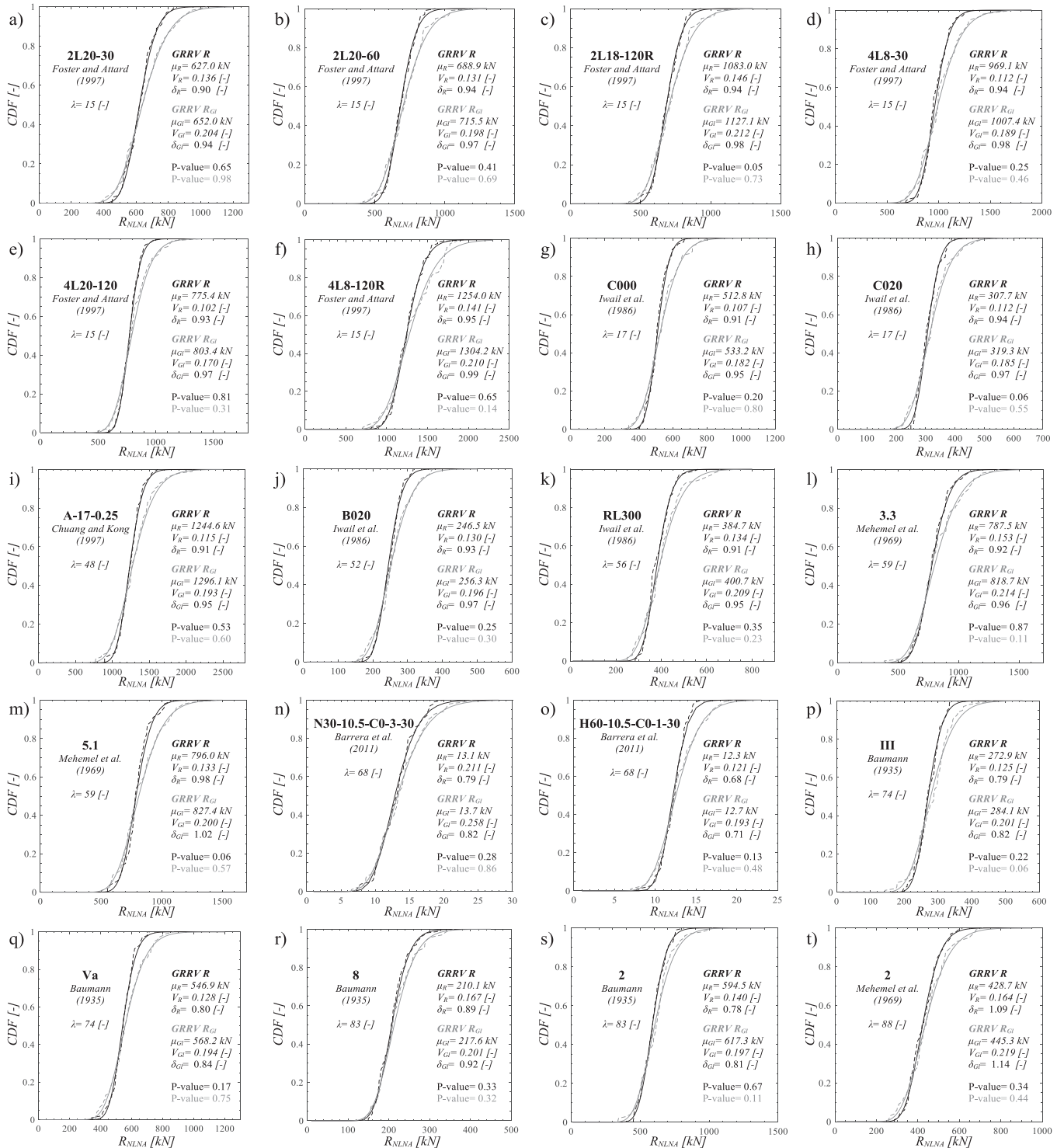
Fig. A1. ‘Empirical’ CDFs and related ‘theoretical’ lognormal CDFs of the GRRVs R and R Gf , fitted by the ML method, for the RC slender members from references [37–45] (slenderness range from 15 to 88).
