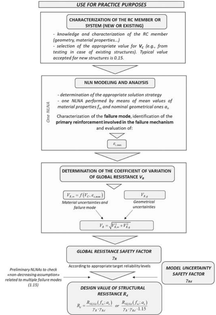
Fig. 2. Proposed calibration philosophy for the novel strain-based approach to assess R_{dI} .
