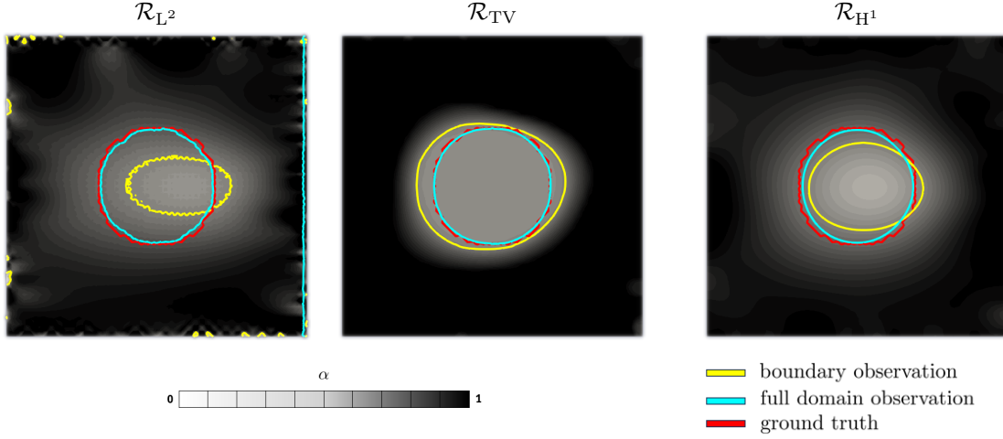
Figure 10: Effect of restricting observations to the boundary. Scar profiles obtained from the minimization of the cost functional (18) with the boundary observation operator for all the possible regularizing terms: \mathcal{R}_{L^2} (left), \mathcal{R}_{TV} (center), and \mathcal{R}_{H^1} (right). Isolines \alpha = 0.4 for the boundary observation (yellow), for the full domain observation (blue) and for the ground truth (red) are superimposed to the contractility pattern. In each case we set \lambda = \lambda_{\text{opt}} . The value of \alpha was rescaled to the range [0, 1] for visual clarity.
