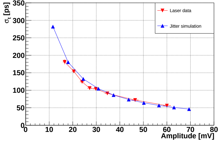
Figure 8. Electronic jitter extracted from circuit simulations (blue) and time resolution from experimental laser measurements (red), acquired with V_{\text{back}} = -30 V and V_{\text{top}} = 40 V.
