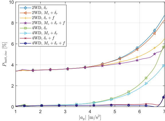
Figure 19 – P_{batt,inc} for the considered actuation configurations along UC iv in Figure 15, for a_x = 1.5 m/s 2 , V = 100 km/h, and \mu_0 = 100\% , w.r.t. the 4WD M_z + \delta_r + f configuration on its energy-efficient UC.
