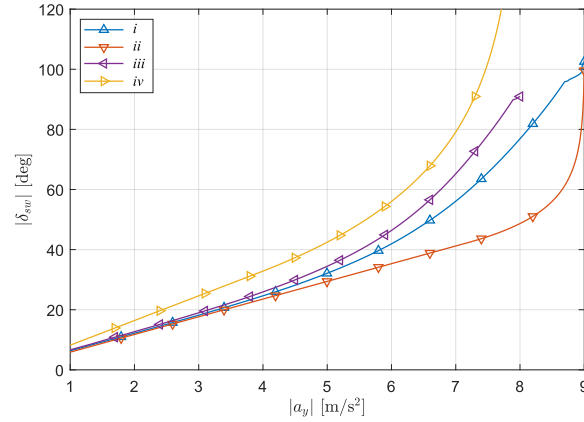
Figure 17 – Selected UCs for V = 100 km/h and \mu_0 = 100\% : i) Characteristic of the baseline 2WD EV at zero a_x ; ii) Sport-oriented characteristic at zero a_x , i.e., with reduced understeer w.r.t. i; iii) Characteristic of the baseline 2WD EV at a_x = 1.5 m/s 2 ; and iv) Stability-oriented characteristic at a_x = 1.5 m/s 2 , i.e., with increased understeer w.r.t. iii.
