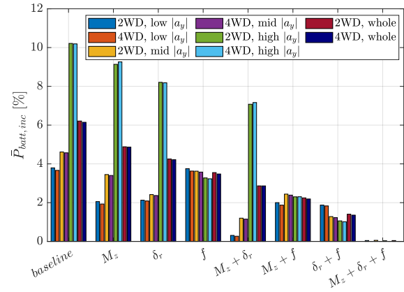
Figure 14 – Summary histograms showing the average battery power increase, \bar{P}_{batt,inc} , w.r.t. the 4WD EV with M_z + \delta_r + f , for bands of lateral acceleration, at zero a_x , V = 100 km/h, and \mu_0 = 100\% . All configurations are operating on their energy-efficient UC.
