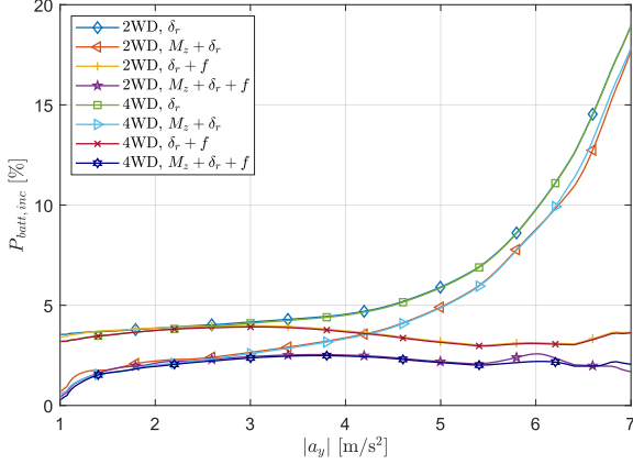
Figure 18 – P_{batt,inc} for the considered actuation configurations along characteristic ii in Figure 15, for zero a_x , V = 100 km/h, and \mu_0 = 100\% , w.r.t. the 4WD M_z + \delta_r + f configuration on its energy-efficient UC.
