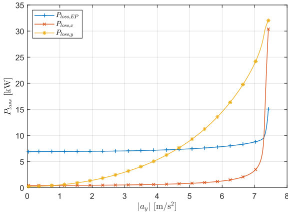
Figure 7 – Power losses during a ramp steer maneuver at a_x = 1.5 \text{ m/s}^2 and V = 100 \text{ km/h} , for the baseline 4WD EV ( M_z = 0 , \delta_r = 0 , and f = 0.68 ), in high tire-road friction conditions.
