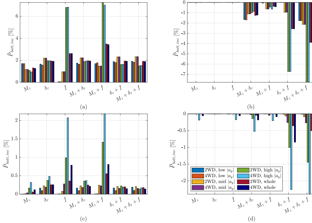
Figure 20 – Summary plots for V = 100 \text{ km/h} and \mu_0 = 100\% . (a) and (b): average battery power increase, \bar{P}_{batt,inc} , while tracking UC i , for zero a_x ; (c) and (d): \bar{P}_{batt,inc} while tracking characteristic iii in Figure 15, for a_x = 1.5 \text{ m/s}^2 . In (a) and (c) the \bar{P}_{batt,inc} value for each set-up is relative to the corresponding 2WD or 4WD configuration tracking the respective energy-efficient UC. In (b) and (d) the \bar{P}_{batt,inc} value for each set-up is relative to the 2WD or 4WD baseline EV.
