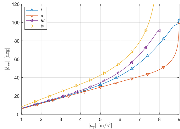
Figure 17 – Selected UCs for V = 100 km/h and \mu_0 = 100\% : i ) Characteristic of the baseline 2WD EV at zero a_x ; ii ) Sport-oriented characteristic at zero a_x , i.e., with reduced understeer w.r.t. i ; iii ) Characteristic of the baseline 2WD EV at a_x = 1.5 m/s 2 ; and iv ) Stability-oriented characteristic at a_x = 1.5 m/s 2 , i.e., with increased understeer w.r.t. iii .
