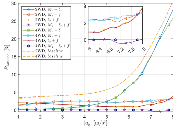
Figure 13 – Relative battery power increase, P_{batt,inc} (in percentage), of the specified actuation configurations ((a) focuses on the single actuator configurations, while (b) focuses on the configurations with multiple actuators), w.r.t. the 4WD EV with M_z + \delta_r + f , at zero a_x , V = 100 km/h, and \mu_0 = 100\% . All configurations are operating on their energy-efficient UC.
