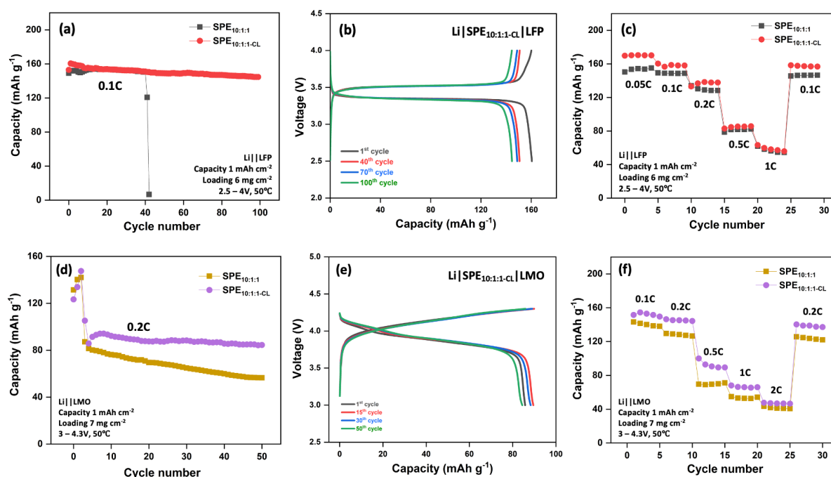
Figure 5. (a) Cycling performance of LFP||Li (active mass loading 6 \text{ mg cm}^{-2} ) cell cycled at 0.1 C rate between 2.5–4.0 V for 100 cycles at 50°C. (b) Charge-discharge profiles of different cycle numbers at 0.1 C rate. (c) Rate performances of LFP||Li cell at different C rates. (d) Cycling performance of LMO||Li (active mass loading 7 \text{ mg cm}^{-2} ) cell cycled at 0.2 C rate between 3–4.3 V for 50 cycles at 50°C. (e) Charge-discharge profiles of different cycle numbers at 0.2 C rate. (f) Rate performances of LMO||Li cell at different C rates.
