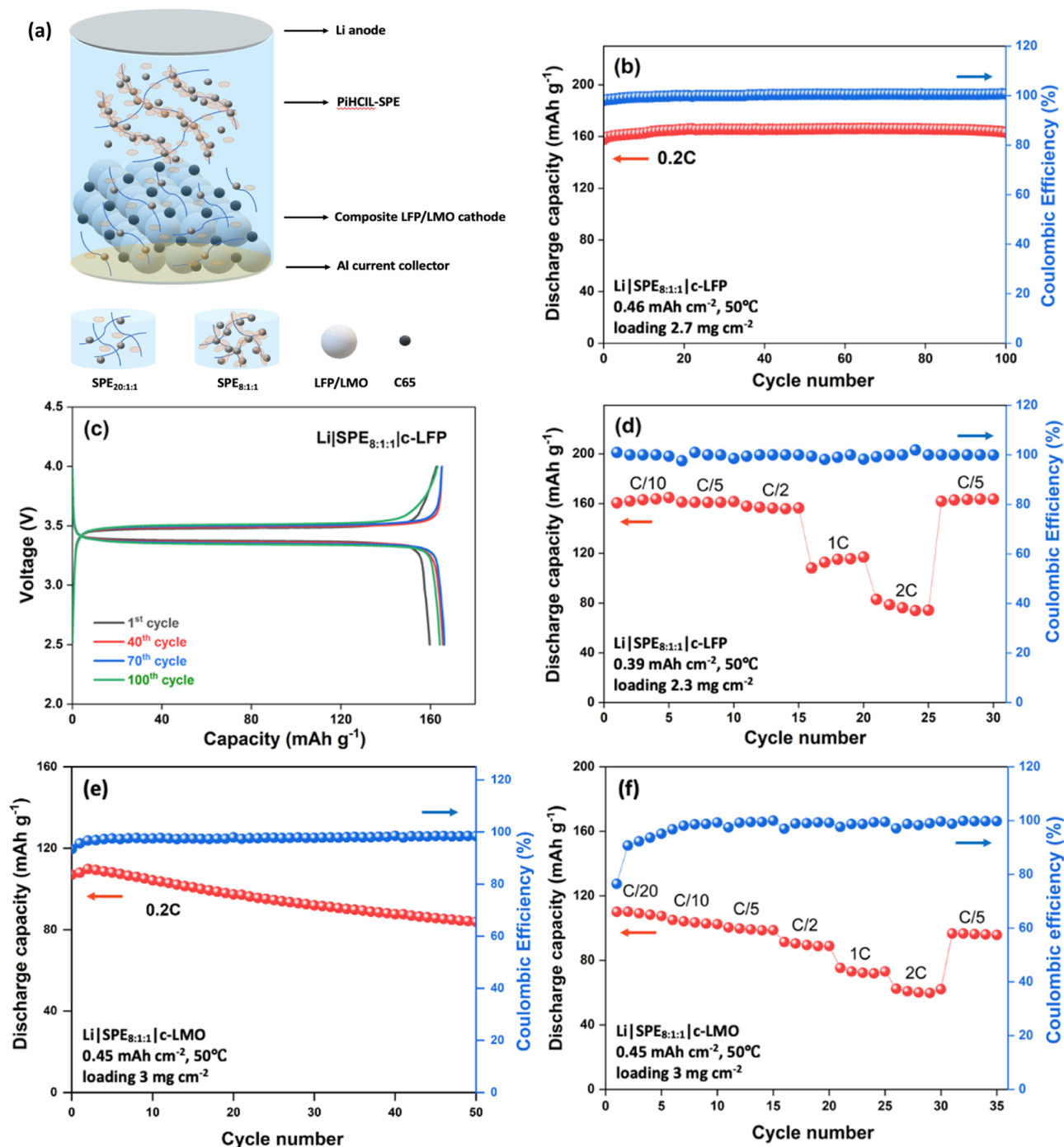
Figure 6. (a) Schematic illustration of the assembled all-solid-state Li|SPE 8:1:1 |c-LFP/c-LMO cell. (b) Cycling performance of Li|SPE 8:1:1 |c-LFP (2.7 mg cm -2 ) cell cycled at C/5 rate (or 0.2 C) between 2.5–4.0 V for 100 cycles. (c) Charge–discharge profiles of different cycle numbers at C/5 rate. (d) Rate performances of Li|SPE 8:1:1 |c-LFP cell (2.3 mg cm -2 ) at different C rates. (e) Cycling performance of Li|SPE 8:1:1 |c-LMO (3 mg cm -2 ) cell cycled at C/5 rate between 3–4.3 V for 50 cycles. (f) Rate performances of Li|SPE 8:1:1 |c-LMO cell (3 mg cm -2 ) at different C rates.
