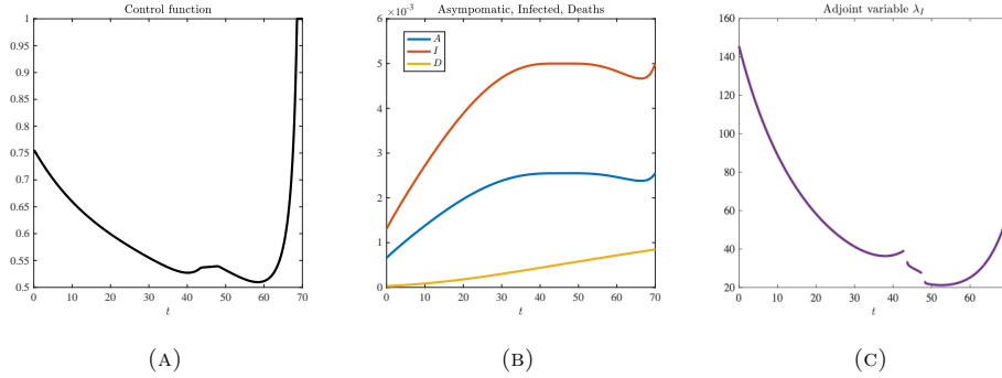
FIGURE 7. Case 2: Solution for T = 70 with state constraint I(t) \leq I_{max} = 0.005 . (A) control u(t) with boundary interval [43.2, 48] . (B) asymptomatics A(t) , infected I(t) and deaths D(t) . (C) adjoint variable \lambda_I(t) .
