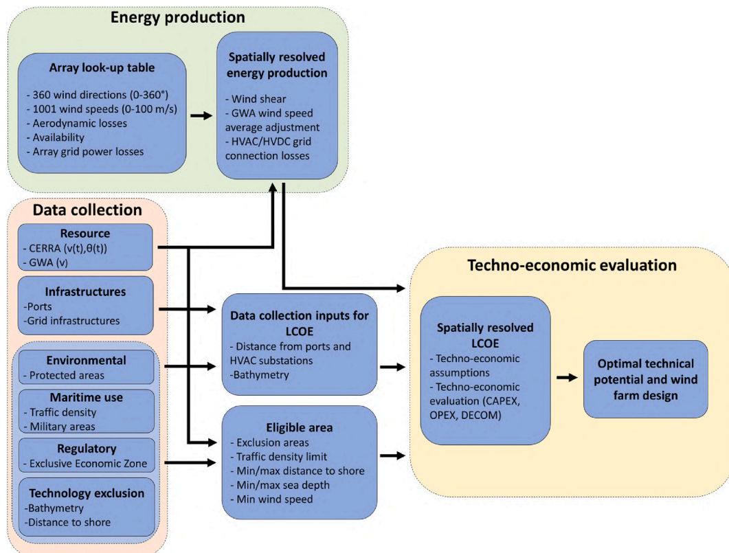
Fig. 1. Methodology to assess the optimal technical potential for Mediterranean countries and the optimal offshore wind farm design. (2-columns image).
