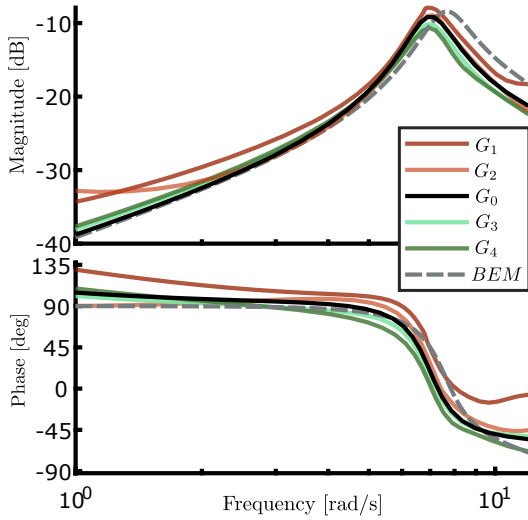
Fig. 5: Comparison of the identified force-to-velocity model depending on the different positions, and BEM response (dashed).
