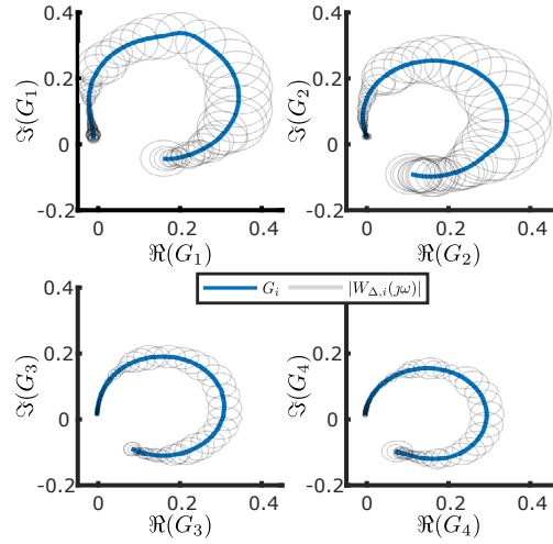
Fig. 6: Uncertainties with respect to the each locking positions.
