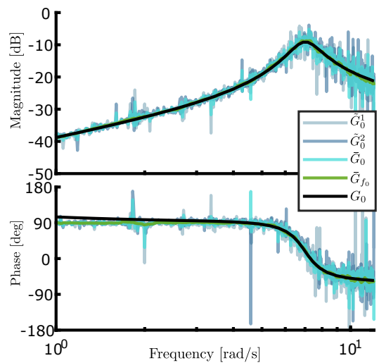
Fig. 4: Identification procedure for the nominal position.
