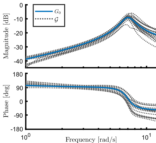
Fig. 8: Defined family \mathcal{G} . The nominal model is indicated with a blue line.
