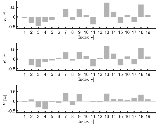
Fig. 9: Power obtained with the system in the set \mathcal{G} for sea-states ISS1,ISS2,ISS3. The index indicates an element considered from the family (5), generated randomly.
