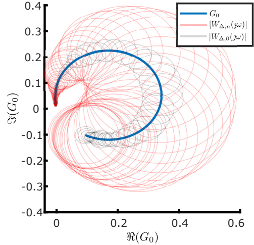
Fig. 7: Uncertainties with respect to the nominal position worst case scenario (red).
