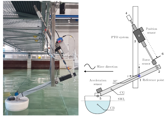
Fig. 1: Photo (left) and schematic illustration (right) of the Wavestar device.
