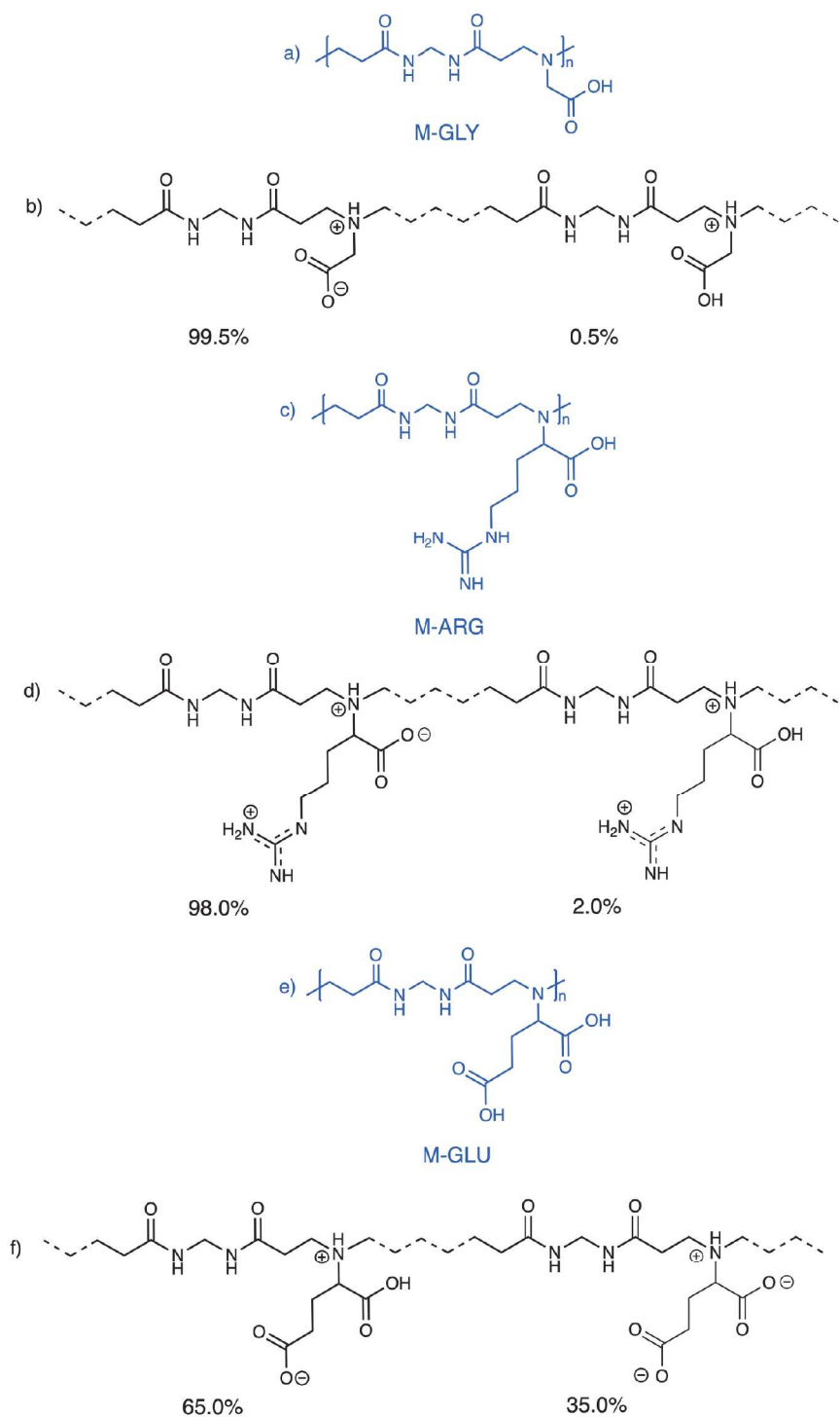
Fig. 1. Repeat units of: M-GLY (a), M-ARG (c) and M-GLU (e). Ionic species distribution at pH 4.0 for: M-GLY (b), M-ARG (d) and M-GLU (f).
