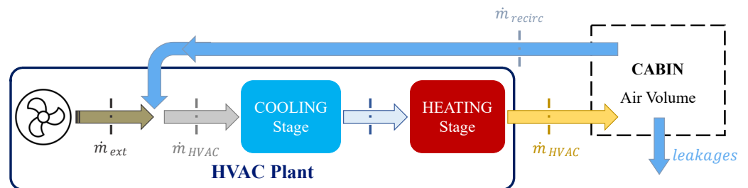
Figure 4. Simplified single-zone HVAC unit scheme.
