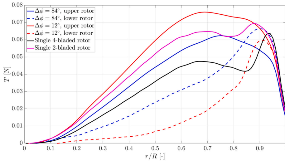
Fig. 11. Comparison of spanwise distribution of thrust between the two co-rotating configuration with \Delta\phi = 84^\circ and 12^\circ and the single 4-bladed and 2-bladed rotors.
