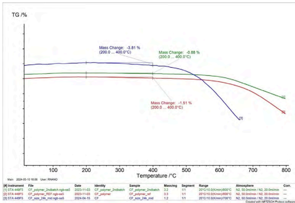
Figure 2. TGA graphs for reference fibres (red line), solvent solvolysed fibres (blue line) and plasma assisted solvolysed fibres (green line). The Y-axis represents weight loss (each bar represents a 20% loss), while the X-axis indicates temperature.
