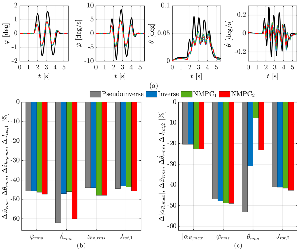
Figure 10. Summary plots for test scenario 3 ((a) time histories of roll angle \varphi , roll rate \dot{\varphi} , pitch angle \theta , and pitch rate \dot{\theta} ; and (b) values of \dot{\varphi}_{rms} , \dot{\theta}_{rms} , \dot{z}_{hv,rms} , and J_{tot,1} ); and for test scenario 4 ((c) values of |\Delta\alpha_{R,max}| , \Delta\dot{\varphi}_{rms} , \Delta\dot{\theta}_{rms} , and \Delta J_{tot,2} ).
