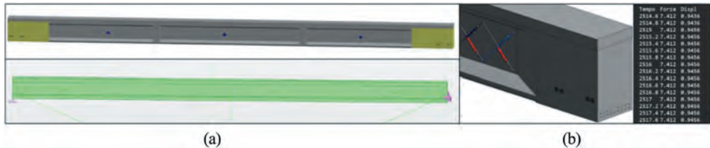
Figure 3. (a) Test families inside beam model and connection with structural model. (b) Sensor detail and link with sensor database.
