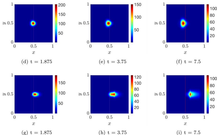
FIG. 5. Test 4. Qualitative evolution of the macroscopic cell density obtained from (2.17)–(2.18)–(2.16) with an initial Gaussian distribution of cells with mean (x_0, y_0) = (0.5, 0.5) and variance \sigma^2 = 10^{-3} . The sensing function is \gamma = \delta(R - \lambda) . The first row refers to the case M_1 in \Omega_1 and M_2 in \Omega_2 , while the second row refers to the case M_2 in \Omega_1 and M_1 in \Omega_2 .
